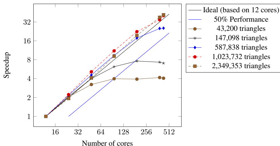
Figure 7.3: Speedups for problems ranging from 43,200 triangles to 2,349,353 triangles showing excellent speedups for the larger problems. We surmise that the super-scalability stems from better cache utilization as the larger meshes are subdivided into smaller meshes that can fit into cache.
