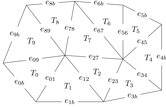
Figure 7.1: Triangular mesh used in our finite volume method. Conserved quantities h , uh and vh are associated with the centroid of each triangular cell, T_i . From the values of the conserved quantities at the centroid of a cell and its neighbouring cells, a discontinuous piecewise linear reconstruction of the conserved quantities is obtained. Fluxes are calculated across each edge e_{ij} using the reconstructed quantities.
