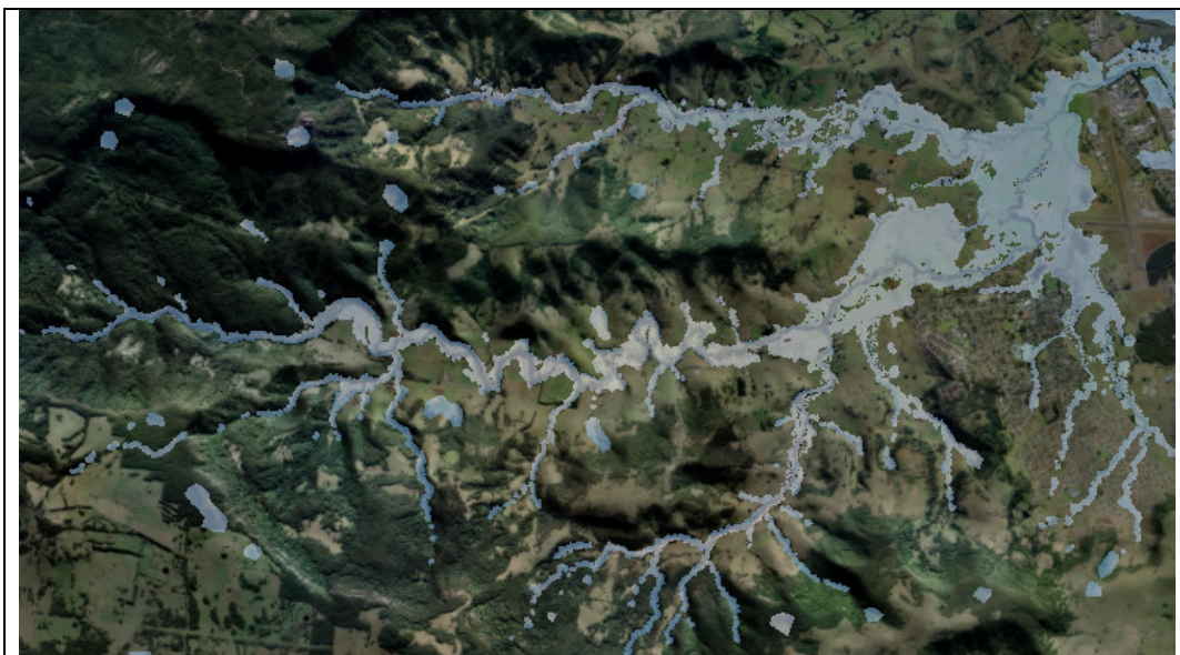
Fig. 8. Entire 110km 2 catchment modelled as a 2D hydrodynamic model using rainfall as input directly onto the computational domain.
