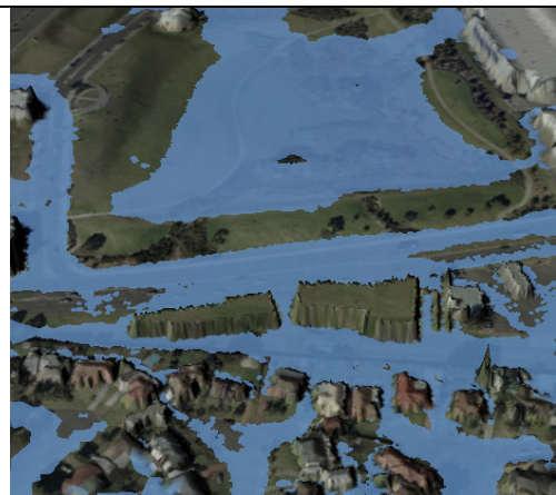
Fig. 9. proposed Post developed inundation (impacting roadway !!)
