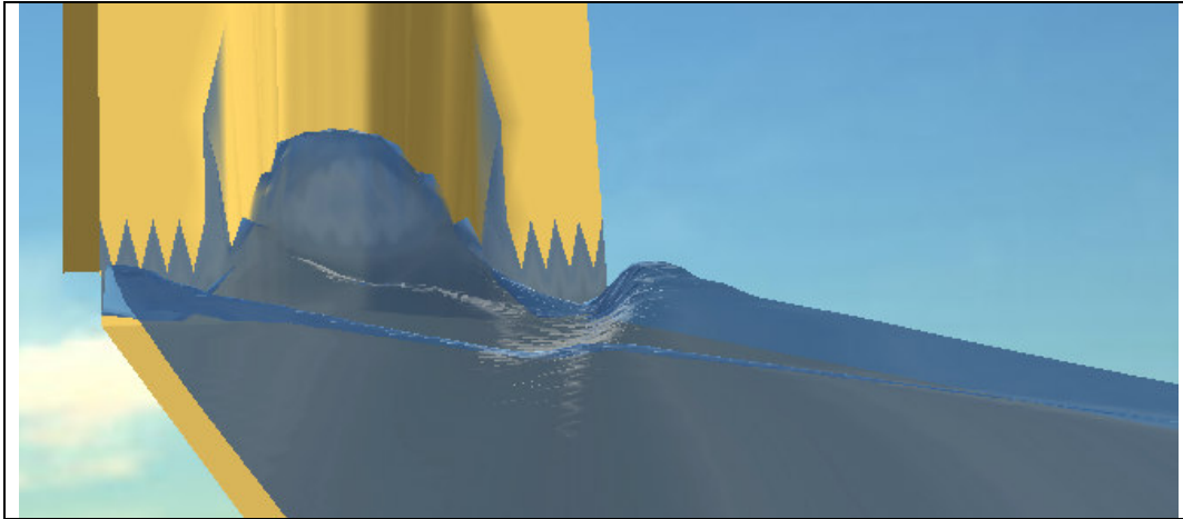
Fig. 7. Detail of the flow leaving a culvert note formation of hydraulic jump
