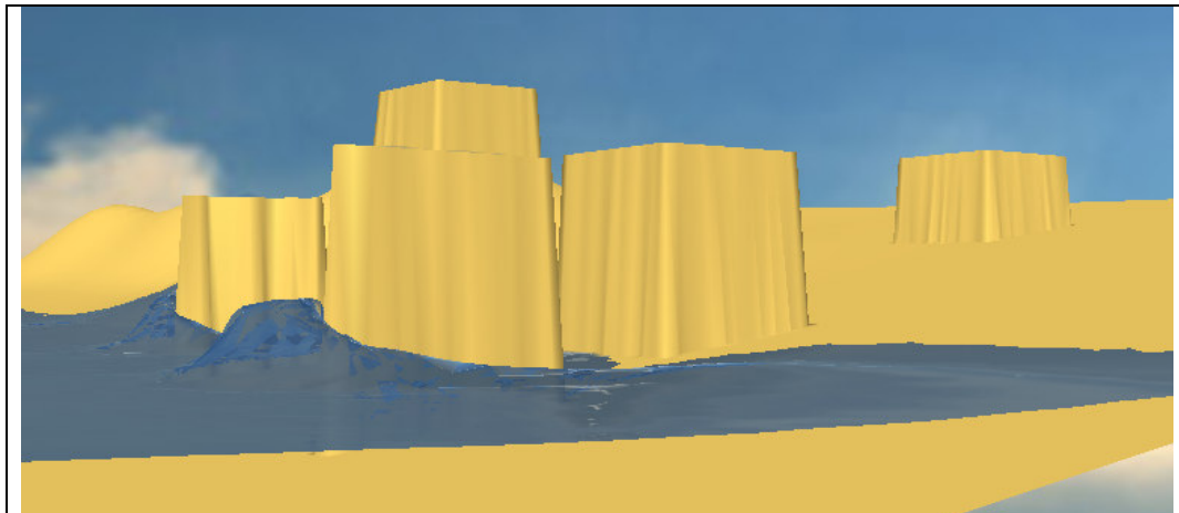
Fig. 4. Anuga handling flow around solid objects in the flow path with the resulting reflective shock wave being formed in front of the building.
