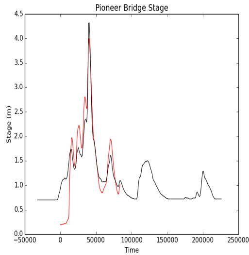
Figure 5.3: Comparison of observed and modelled stage near a bridge in the towradgi simulation
